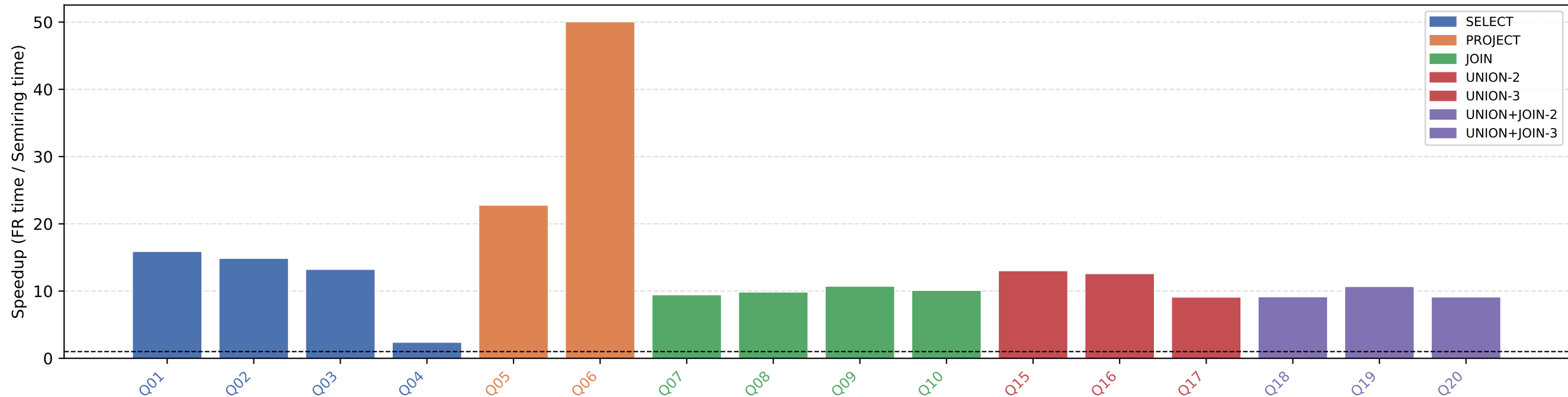
Semiring Speedup over Firing Rules (FR / How-Provenance)
