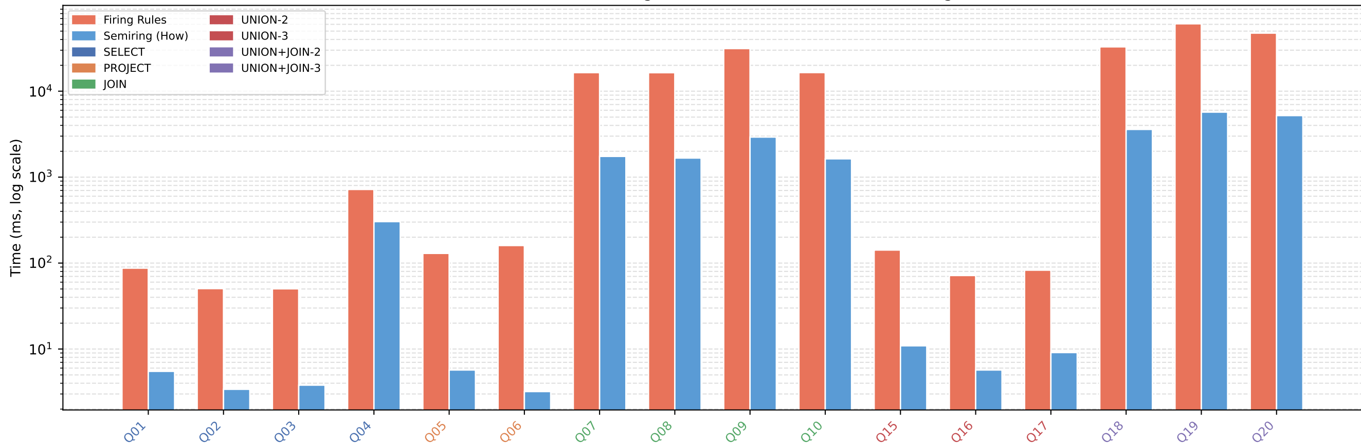
Execution Time: Firing Rules vs. How-Provenance Semiring
