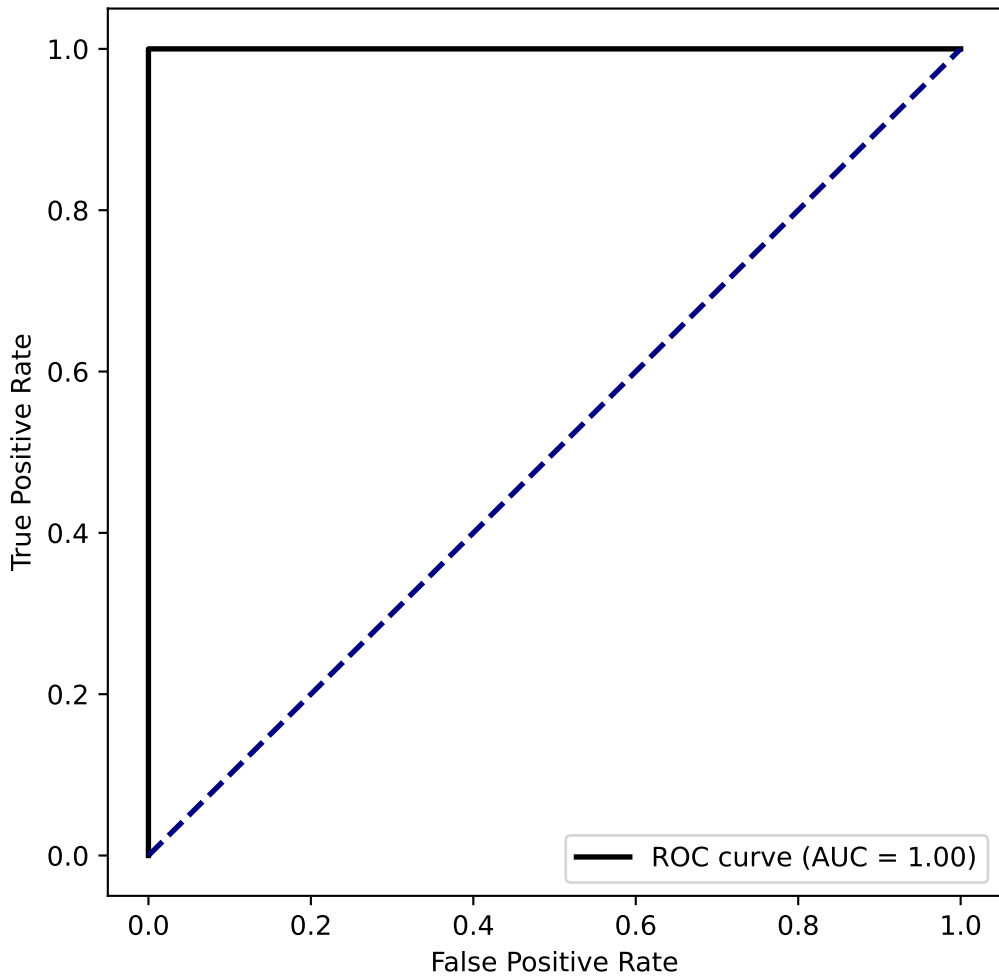
ROC Curve - Detecting tumor sample in HNSCC in testing set
