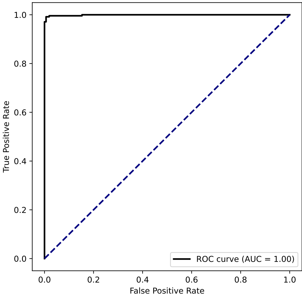
ROC Curve - Detecting tumor sample in combined in testing set
