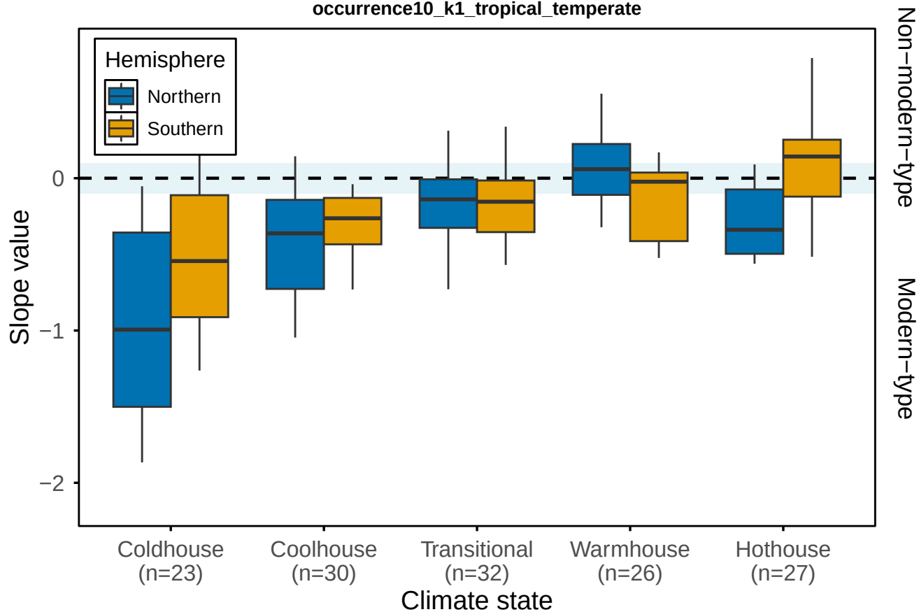
percentile_latbin_OLS | q75 occurrence10_k1_tropical_temperate
