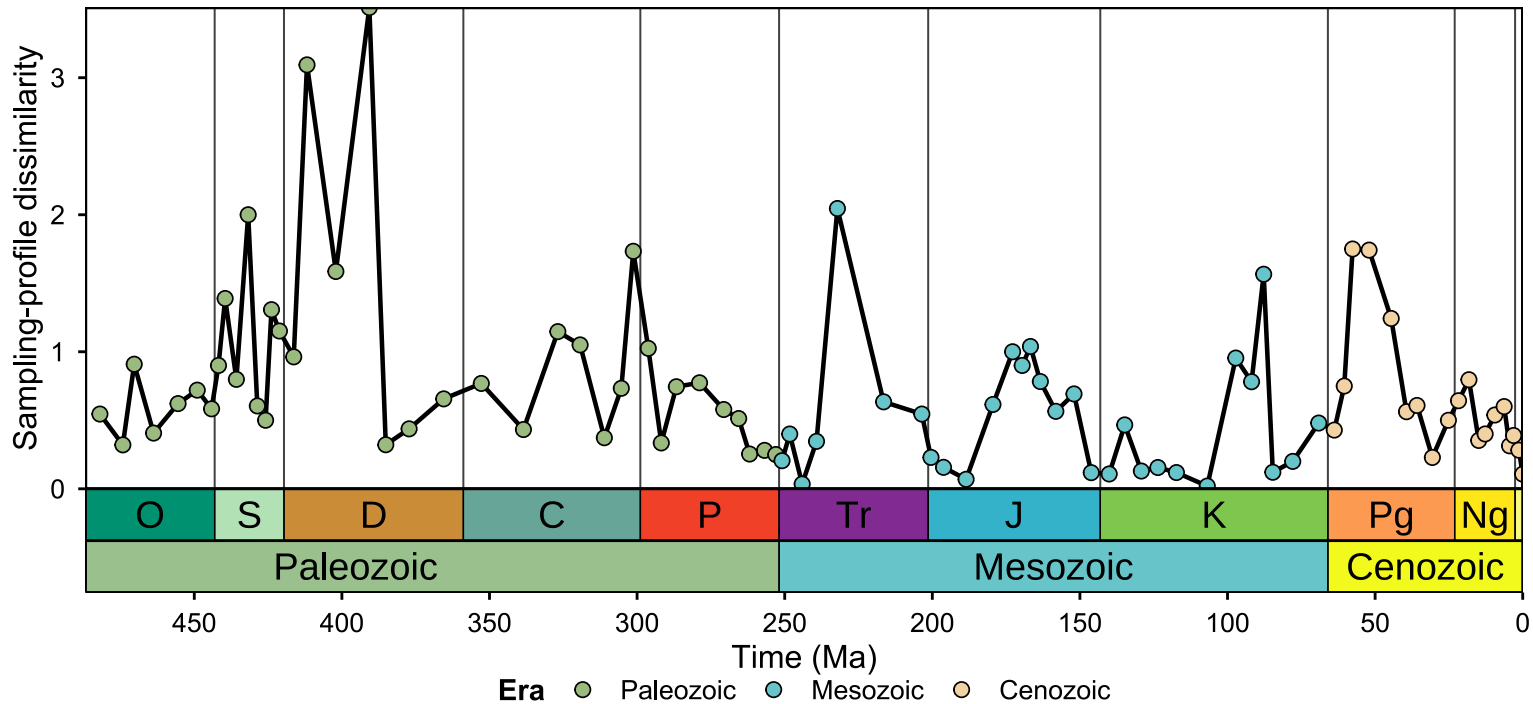
NH-SH sampling-profile dissimilarity | occurrence5_k1_tropical_temperate
