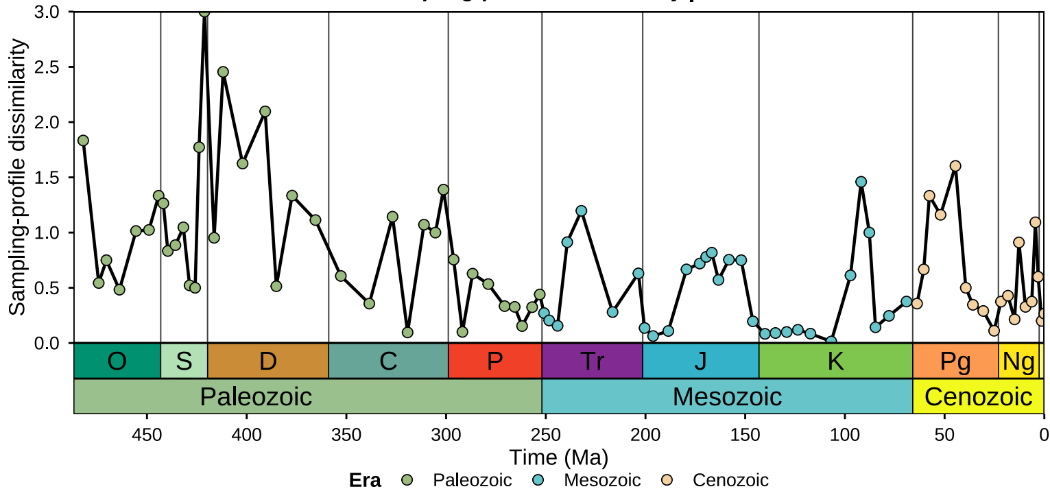
NH-SH sampling-profile dissimilarity | collection5
