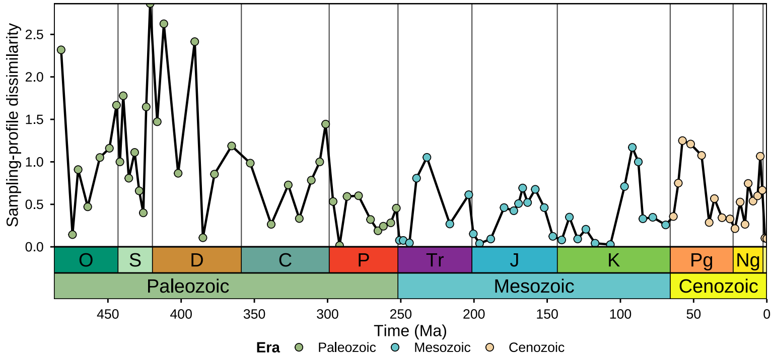
NH-SH sampling-profile dissimilarity | occurrence5
