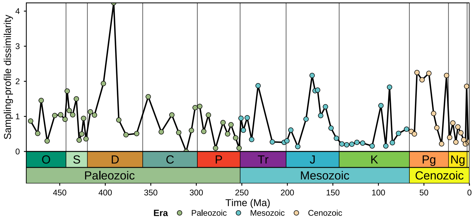
NH-SH sampling-profile dissimilarity | occurrence10
