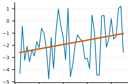
South Dakota +0.06 °C/dec (SE 0.29)
