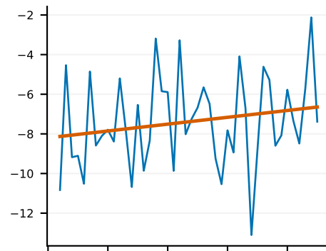
Wisconsin +0.35 °C/dec (SE 0.27)
