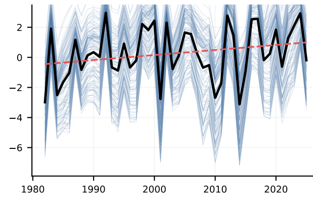
09_descriptive_weather_full
