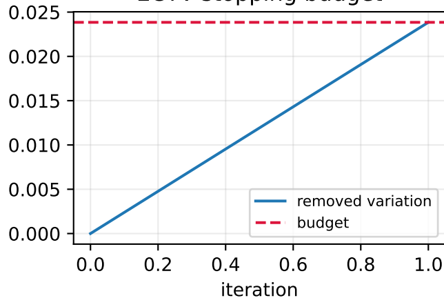
ECTV stopping budget
