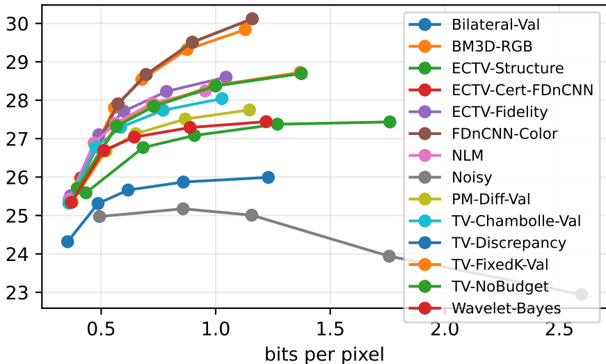
PSNR after JPEG
