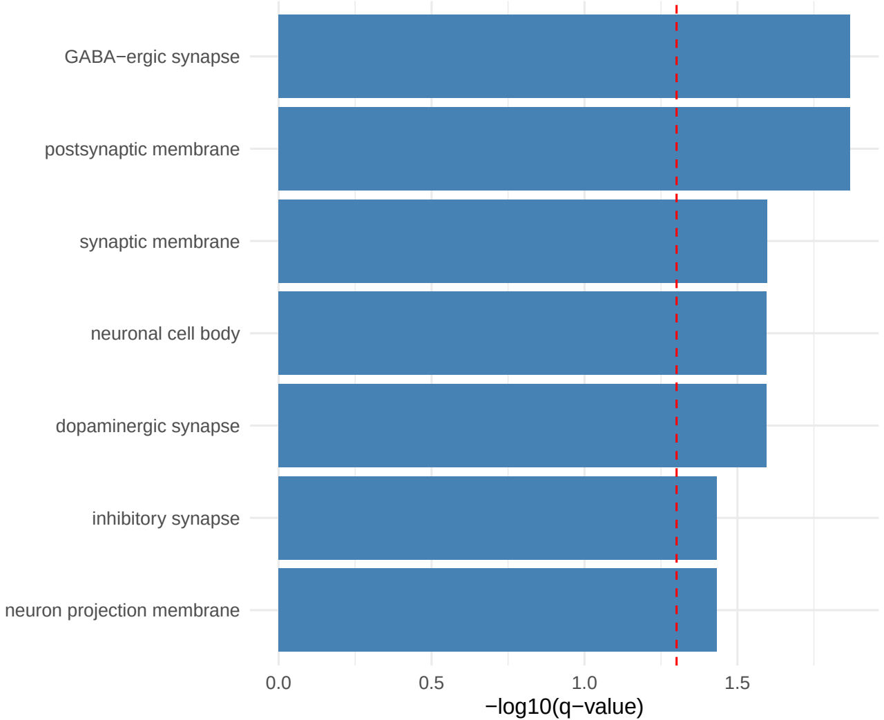
Pattern 13 Top Enriched GO Terms
