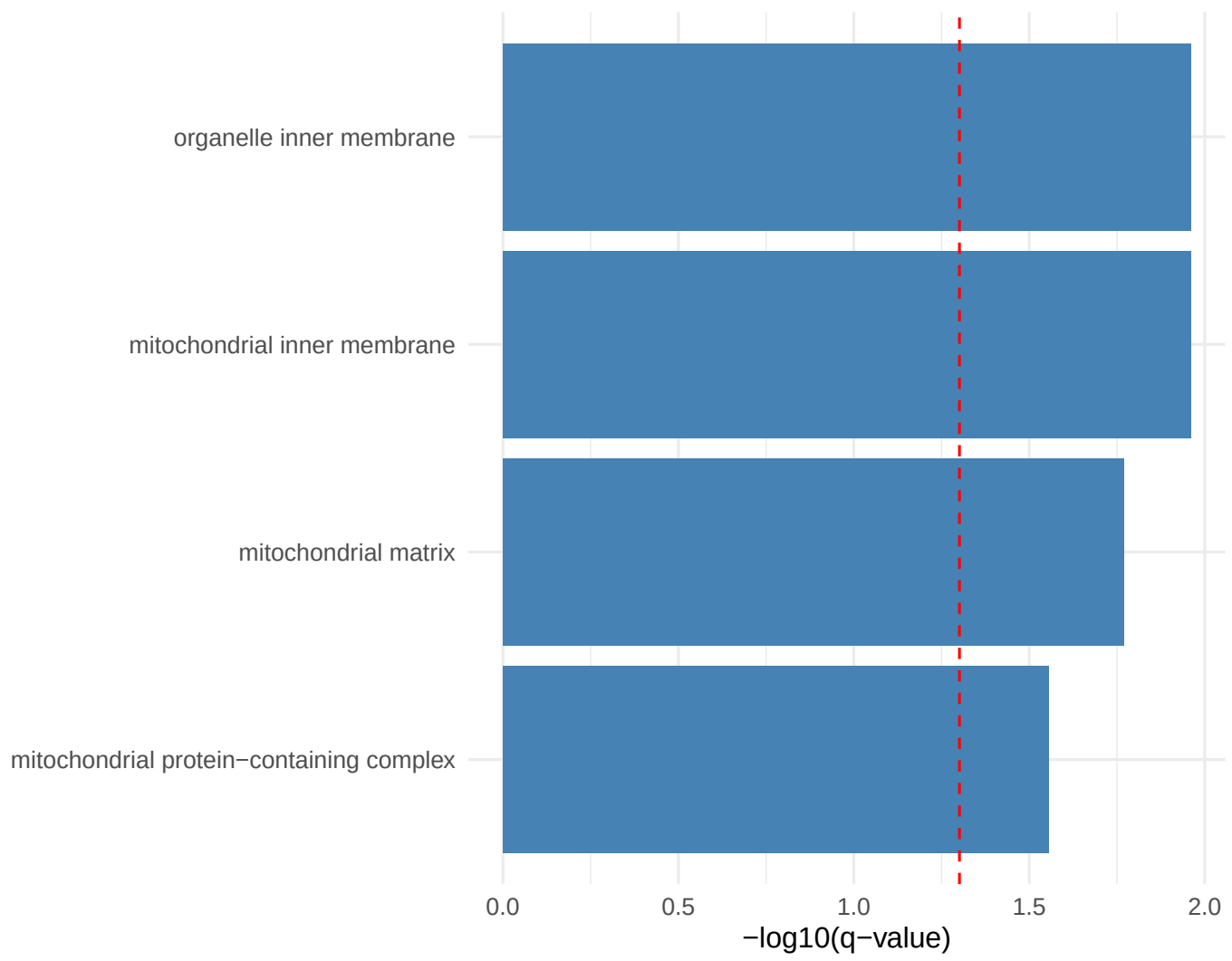
Pattern 14 Top Enriched GO Terms
