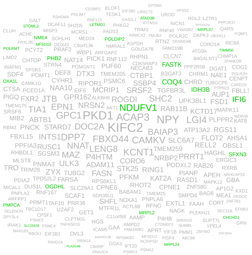
Pattern 14 Genes Highlighted by GO
