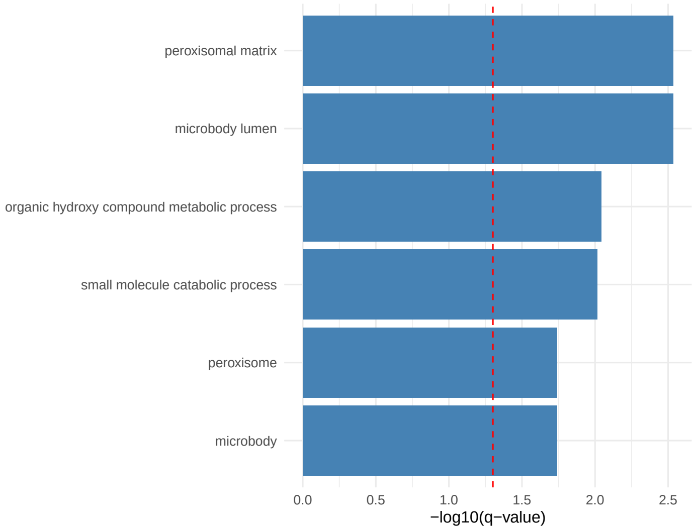
Pattern 15 Top Enriched GO Terms
