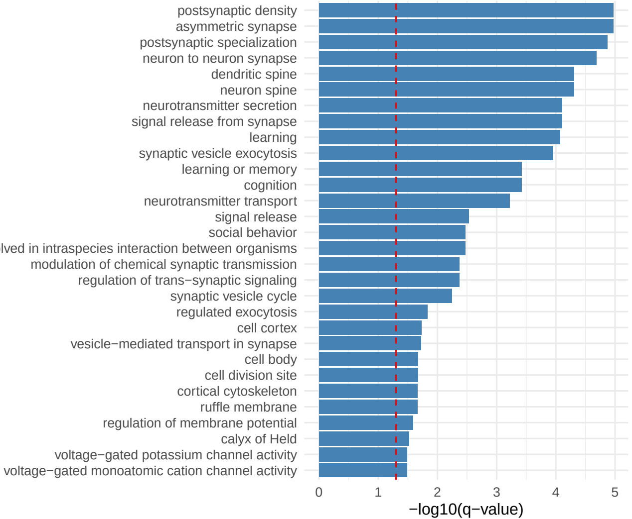
Pattern 23 Top Enriched GO Terms
