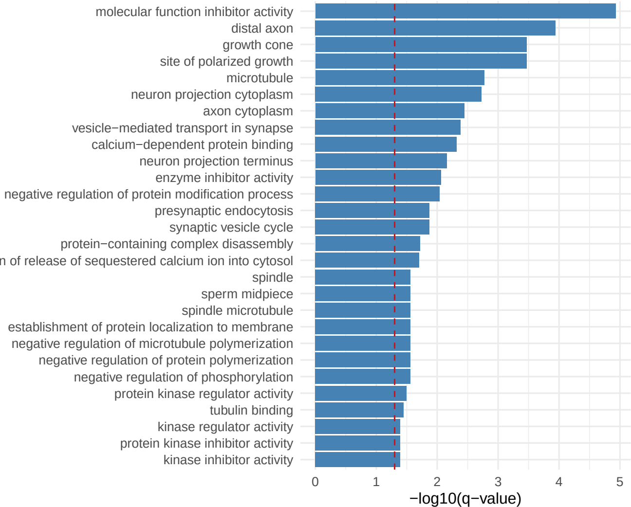
Pattern 45 Top Enriched GO Terms
