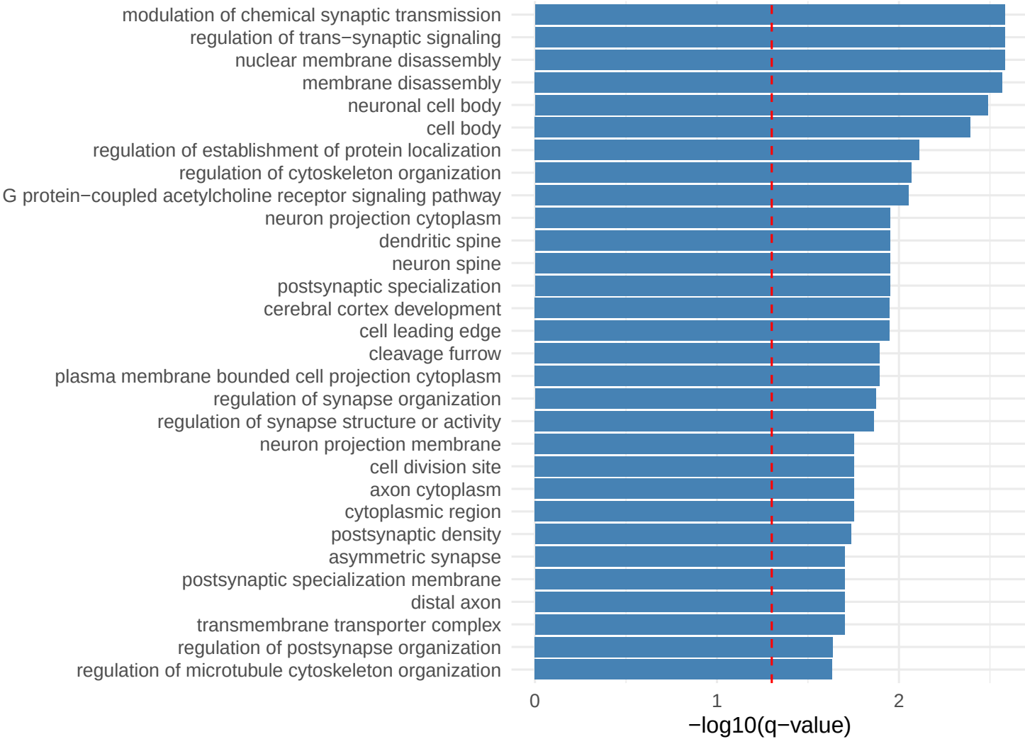
Pattern 46 Top Enriched GO Terms
