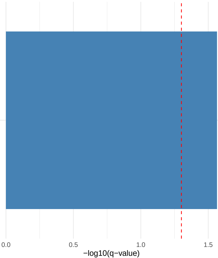
Pattern 47 Top Enriched GO Terms
