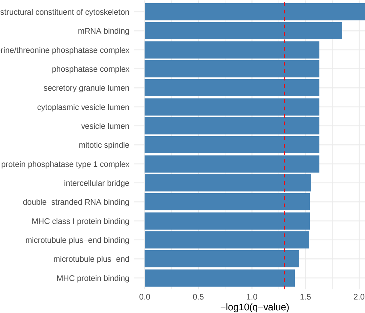
Pattern 72 Top Enriched GO Terms
