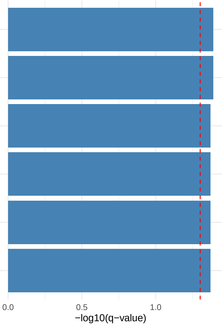
Pattern 76 Top Enriched GO Terms
