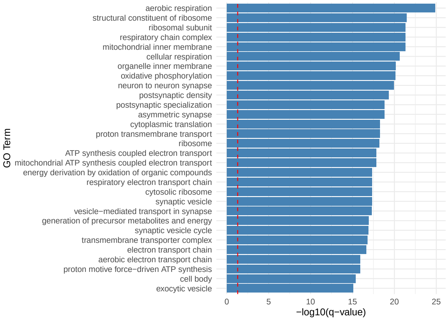
Pattern 14 Top Enriched GO Terms
