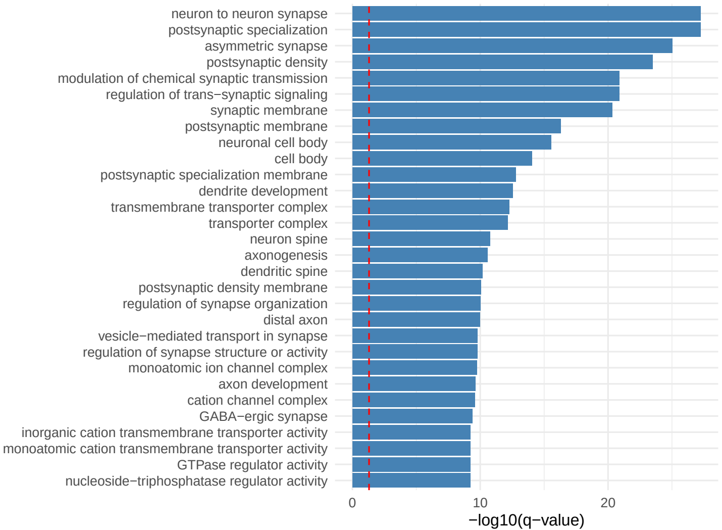
Pattern 18 Top Enriched GO Terms
