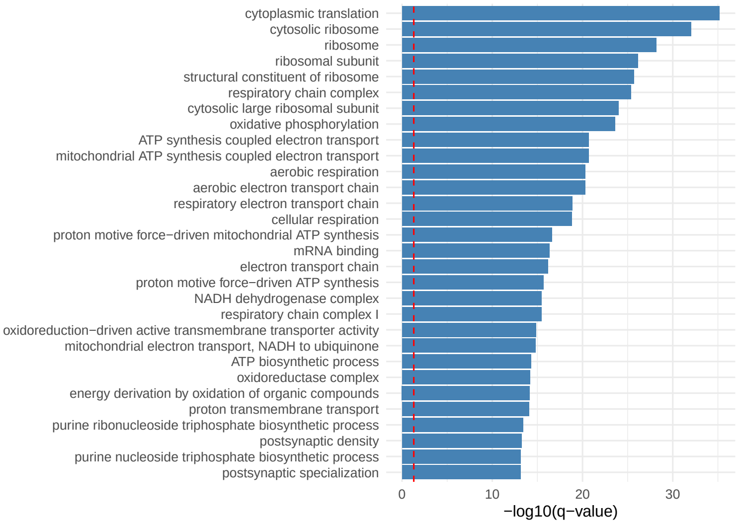
Pattern 20 Top Enriched GO Terms
