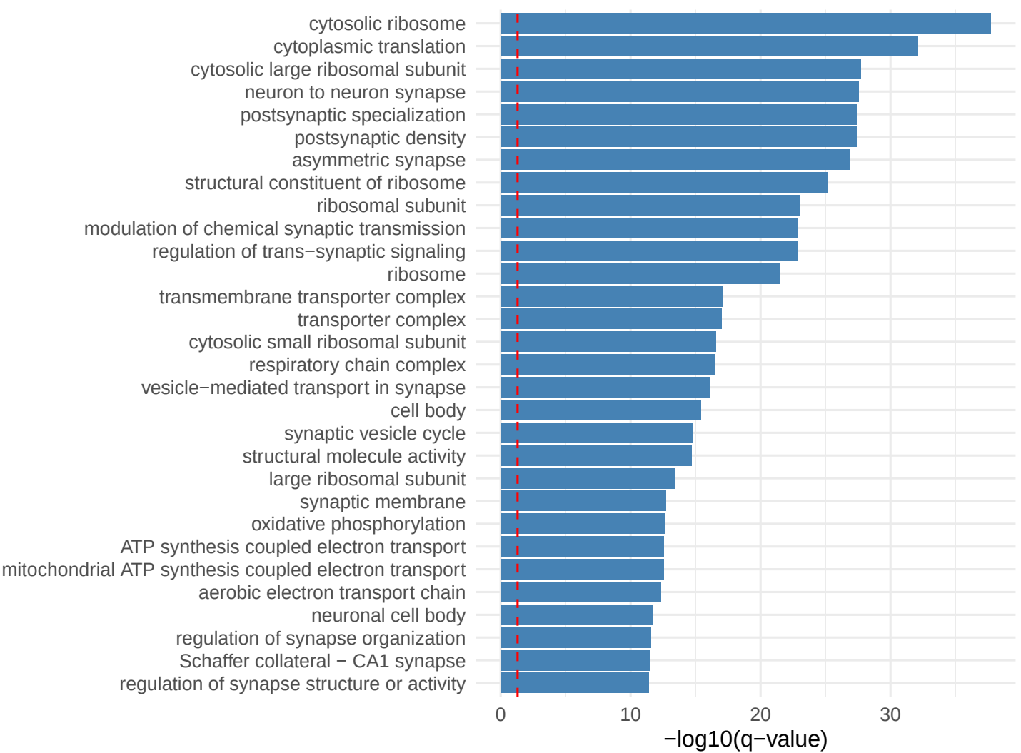
Pattern 23 Top Enriched GO Terms
