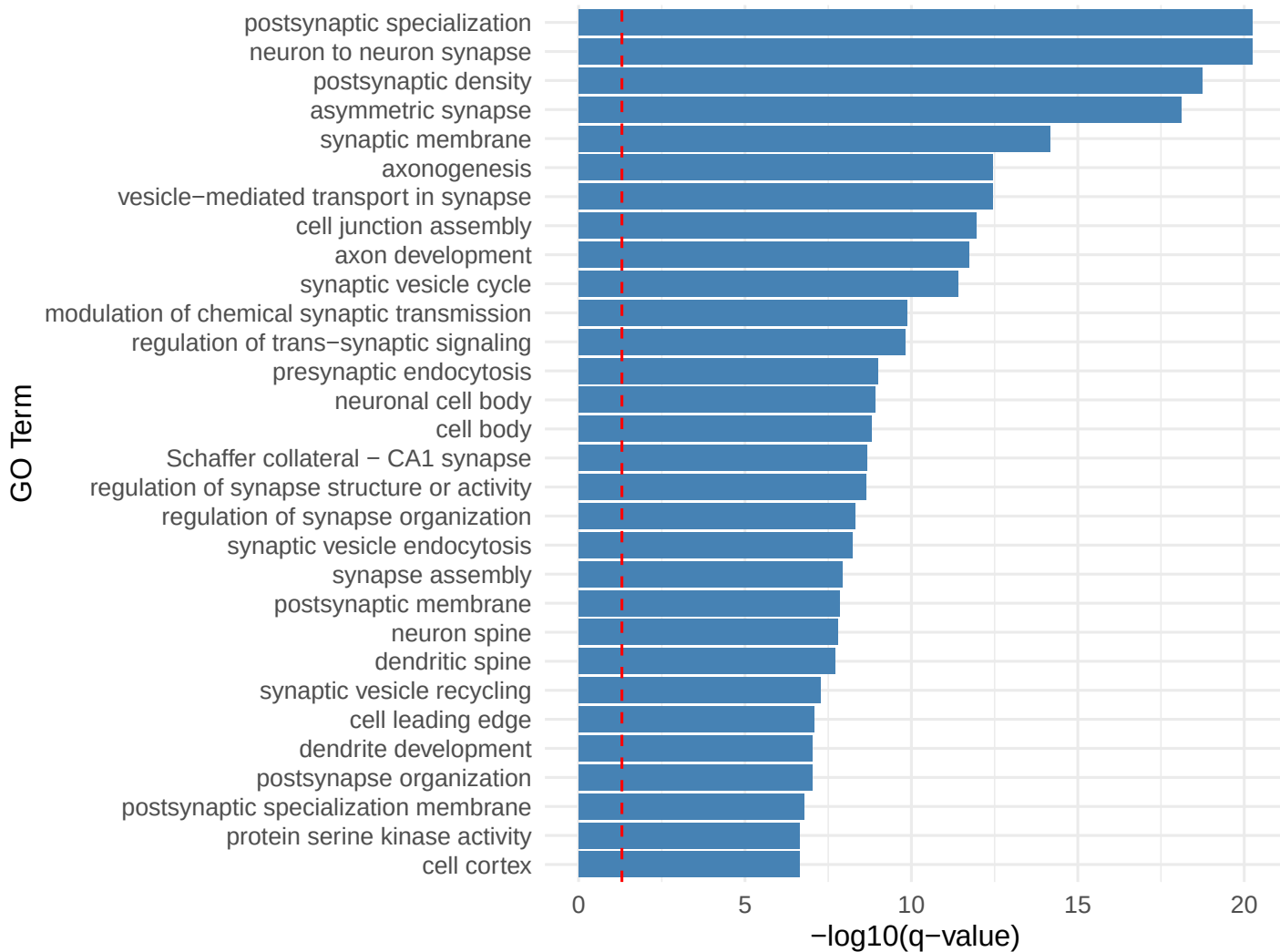
Pattern 32 Top Enriched GO Terms
