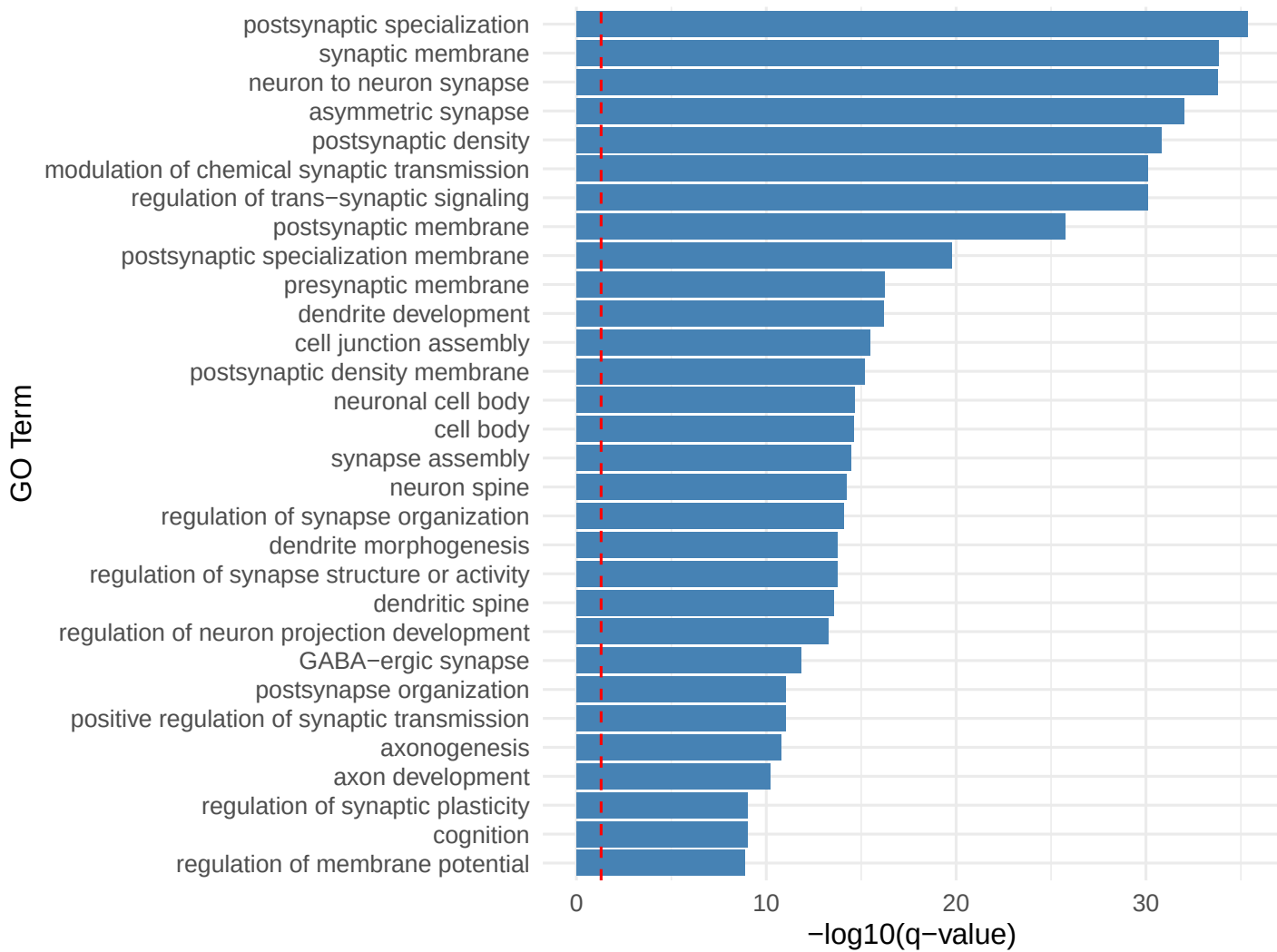
Pattern 44 Top Enriched GO Terms
