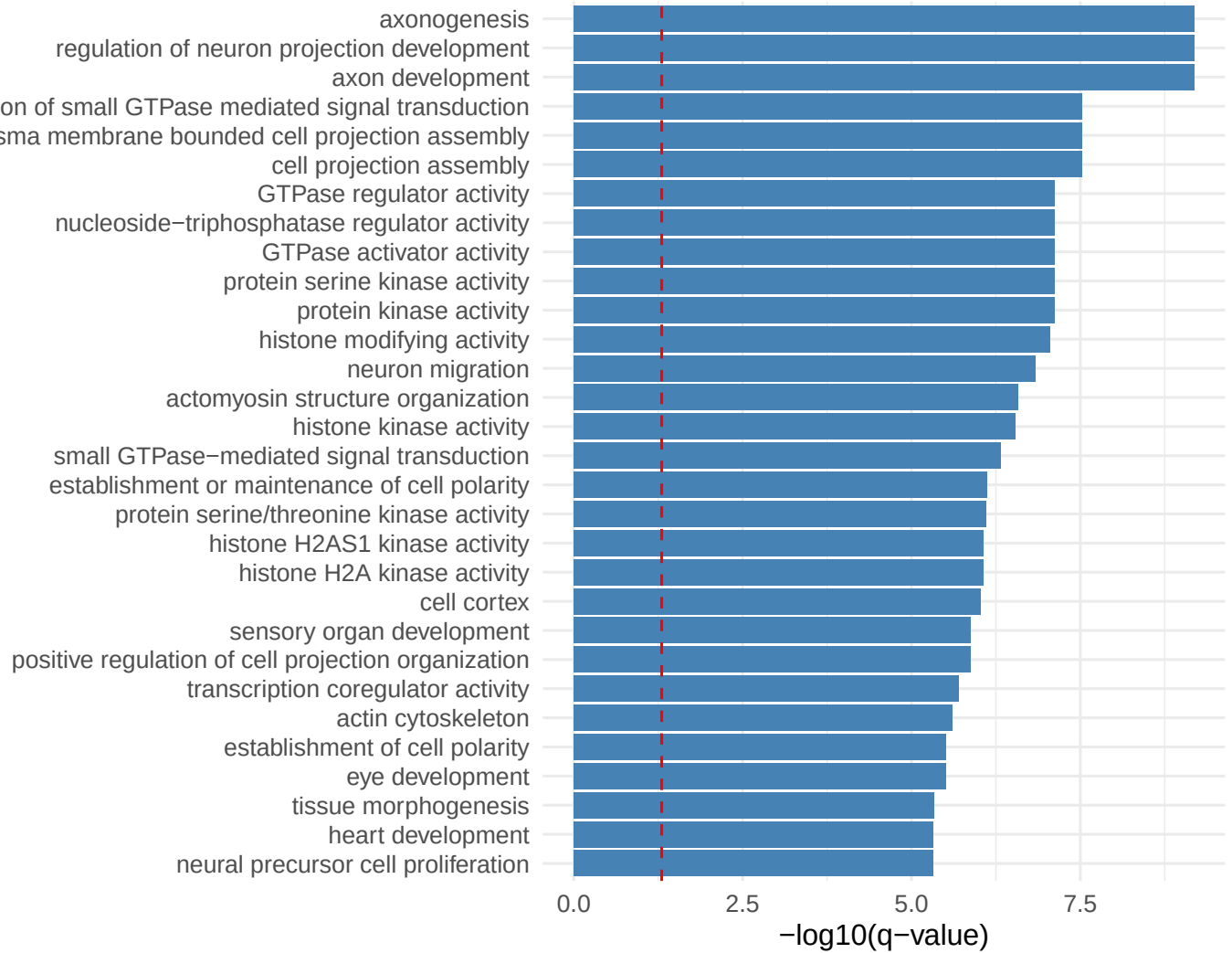
Pattern 50 Top Enriched GO Terms
