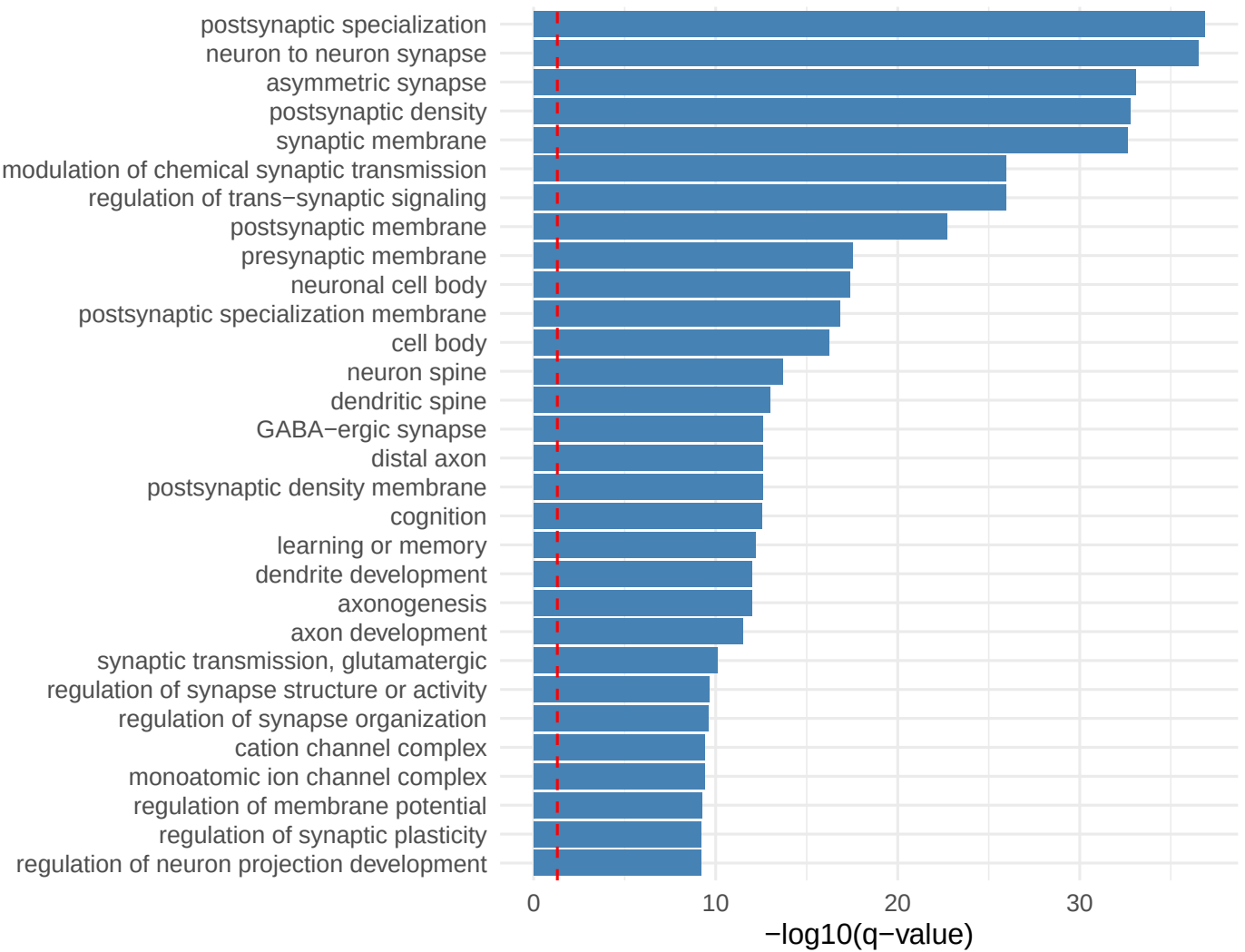
Pattern 54 Top Enriched GO Terms
