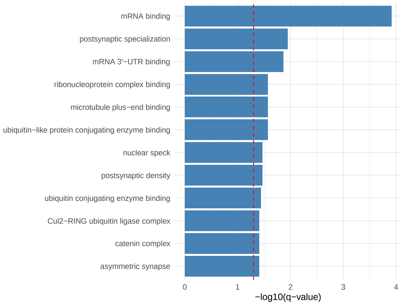
Pattern 57 Top Enriched GO Terms
