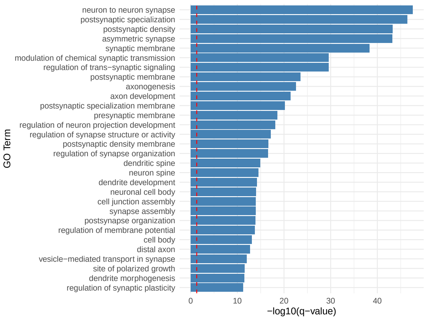
Pattern 59 Top Enriched GO Terms
