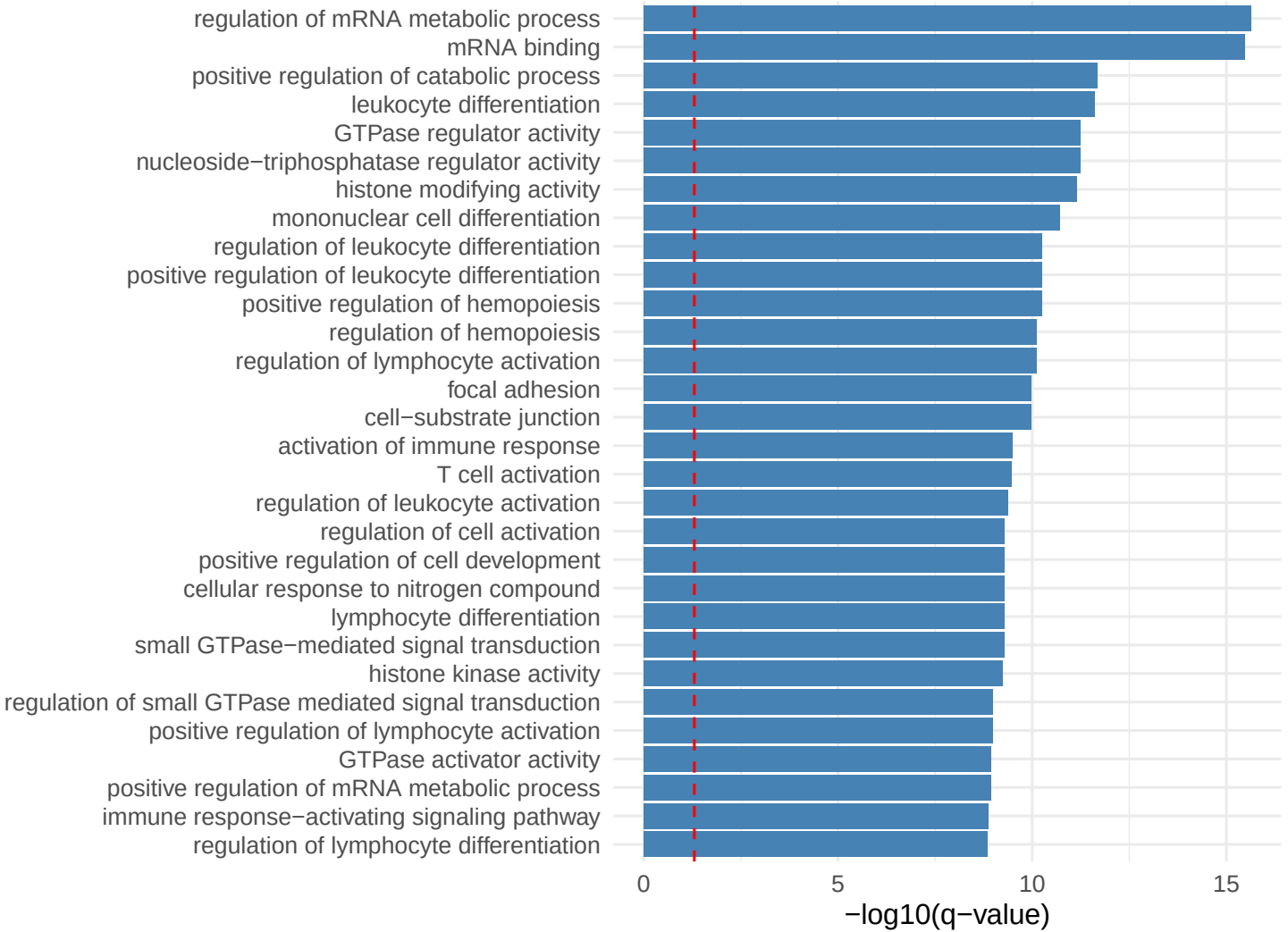
Pattern 78 Top Enriched GO Terms
