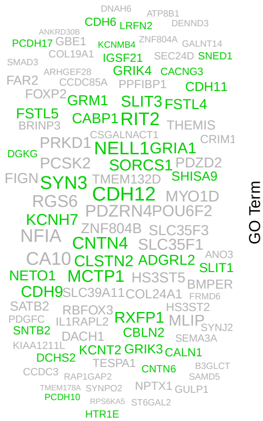
Pattern 30 Genes Highlighted by GO
