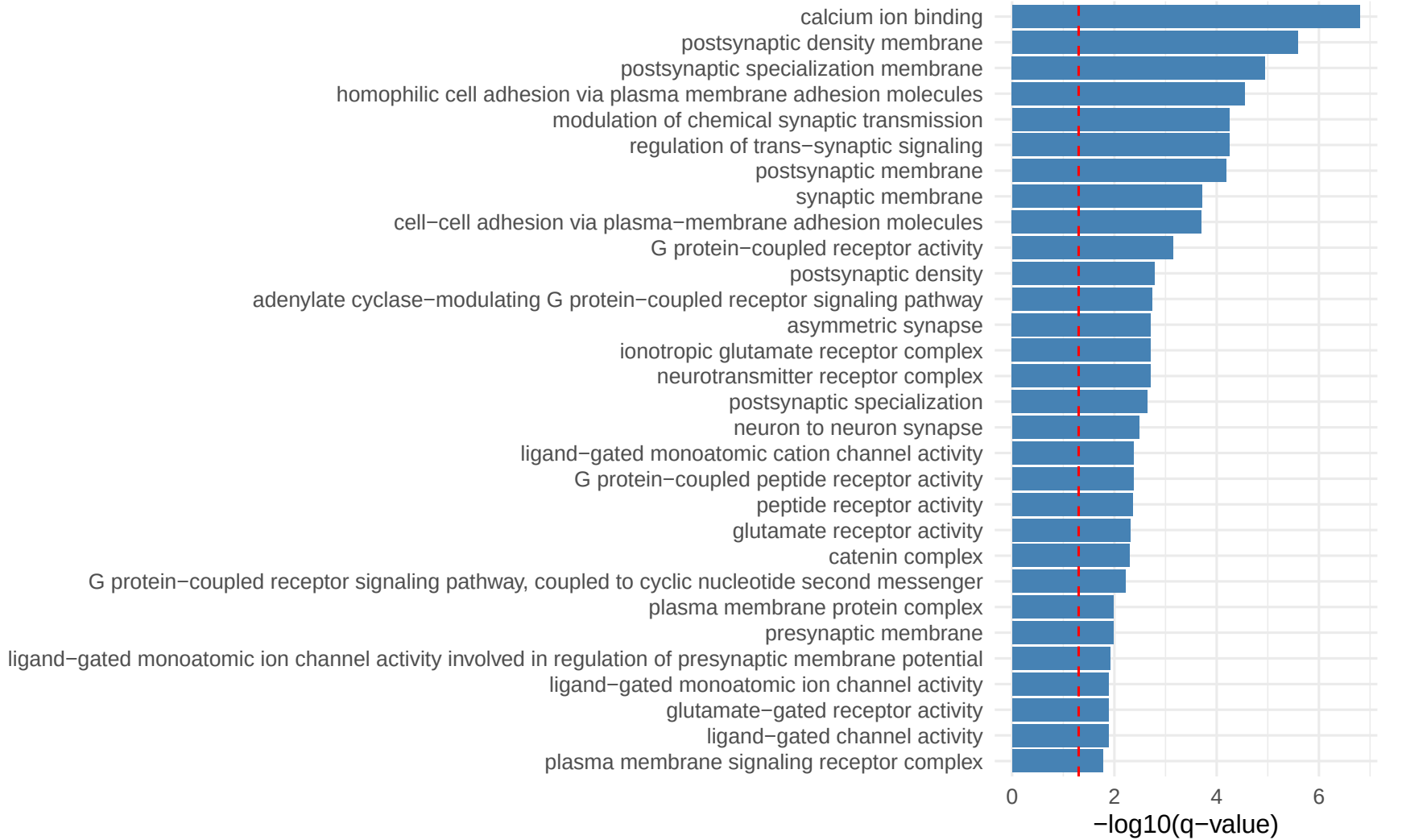
Pattern 30 Top Enriched GO Terms
