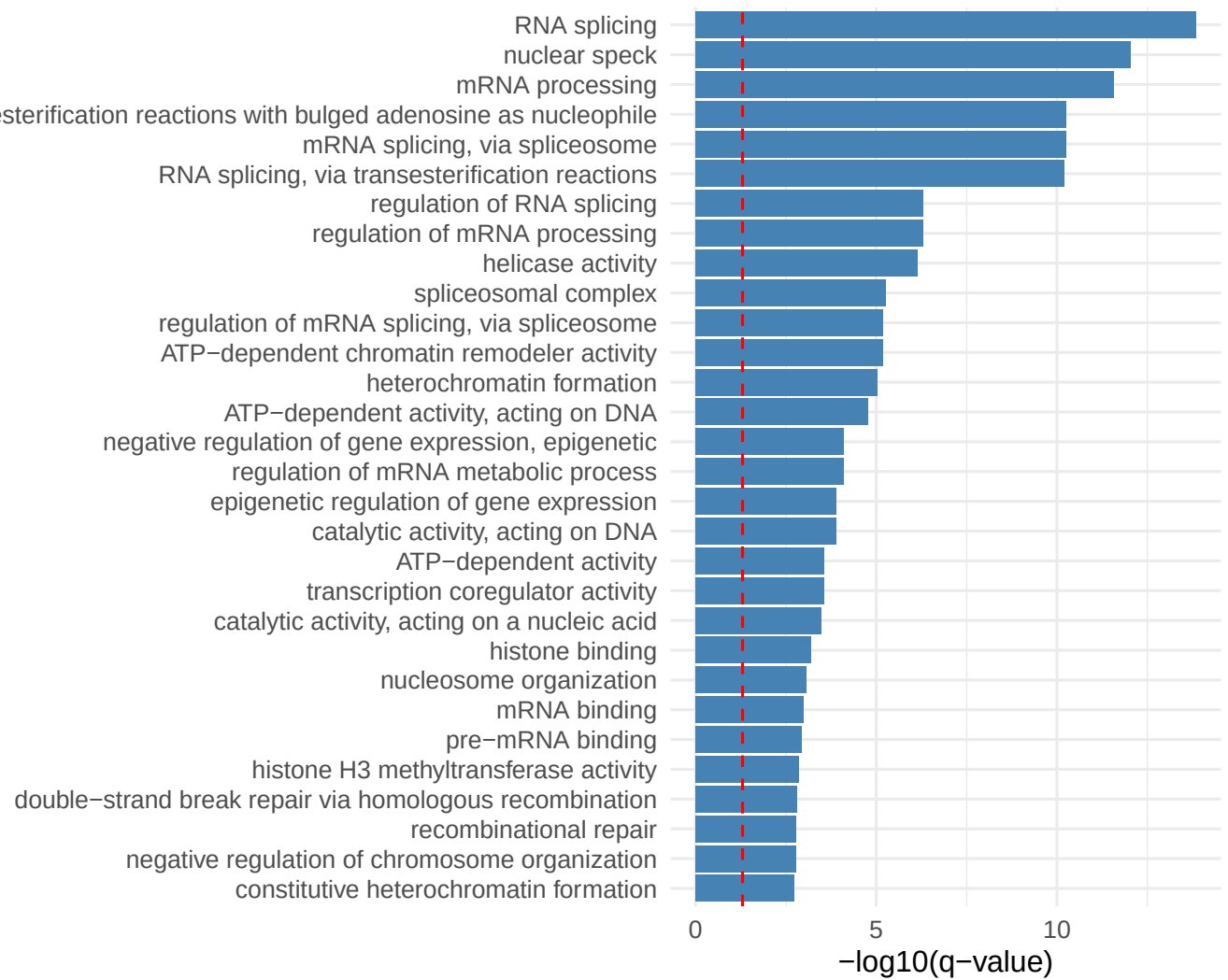
Pattern 33 Top Enriched GO Terms
