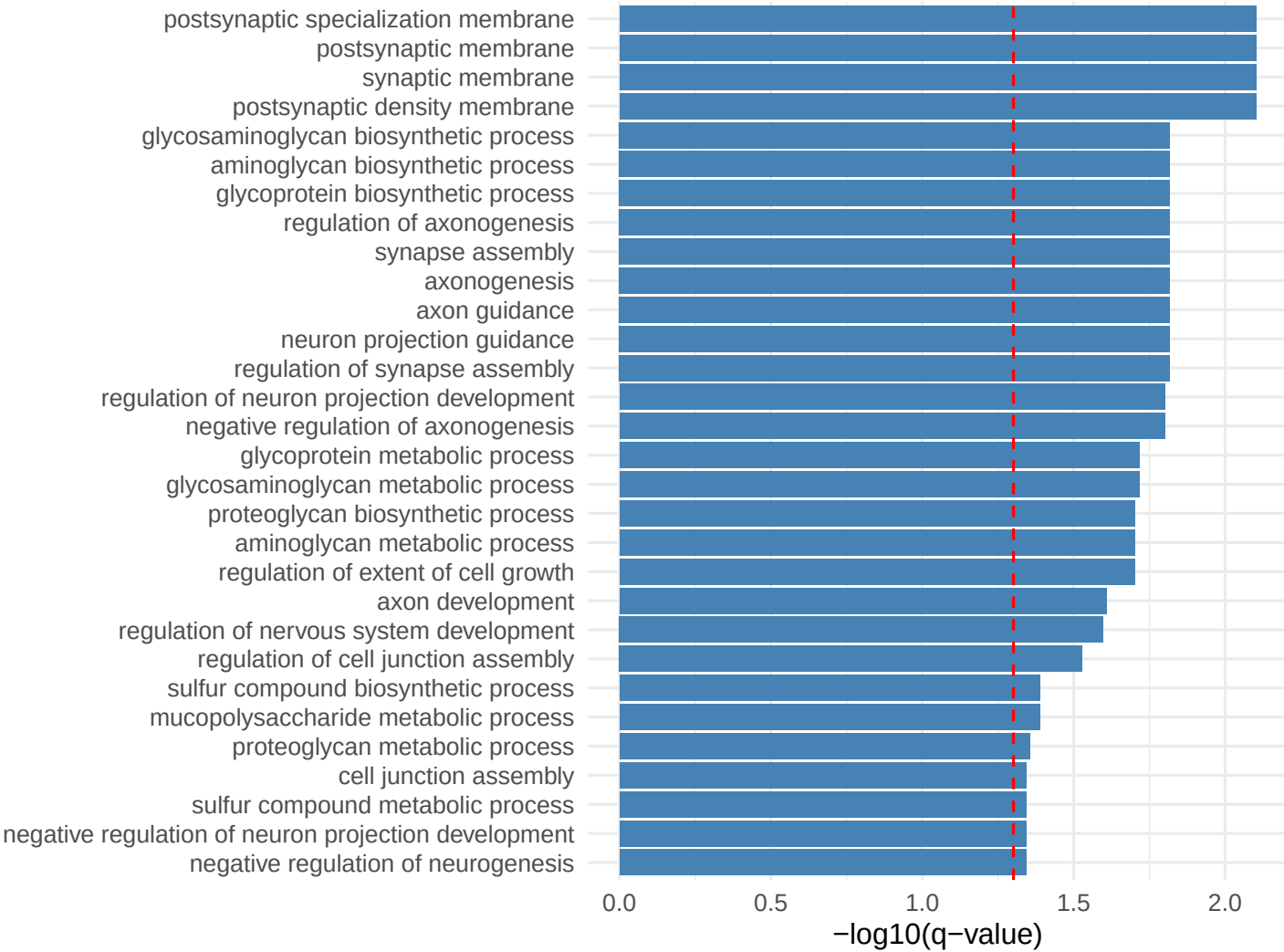
Pattern 36 Top Enriched GO Terms
