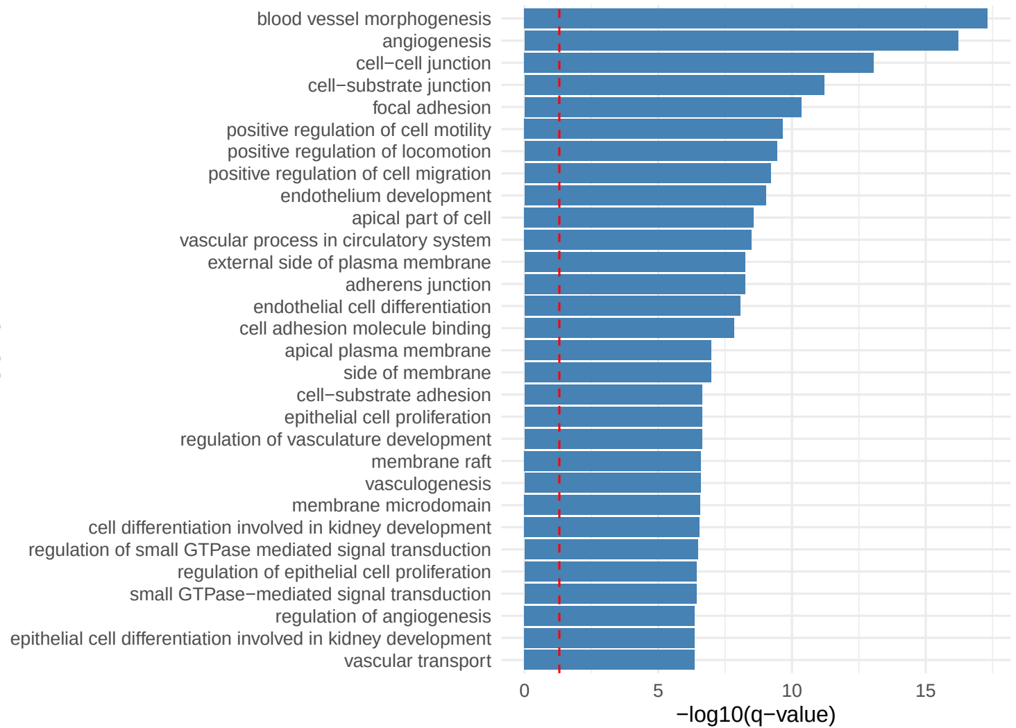
Pattern 39 Top Enriched GO Terms
