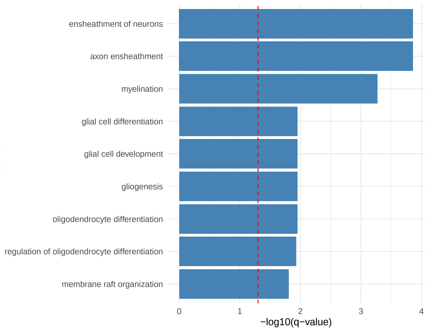
Pattern 3 Top Enriched GO Terms
