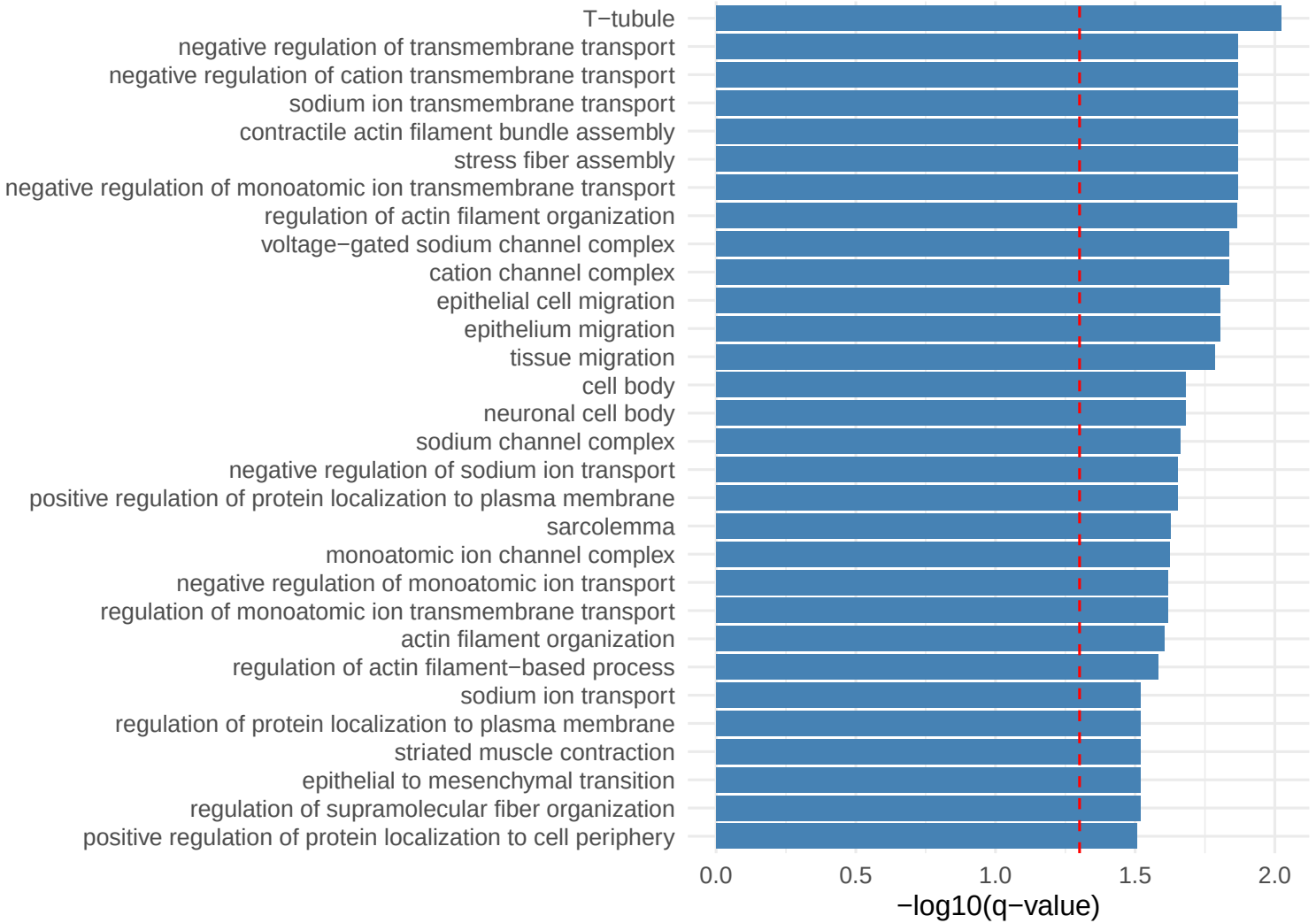
Pattern 40 Top Enriched GO Terms
