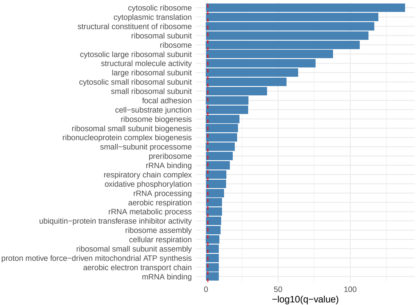
Pattern 41 Top Enriched GO Terms
