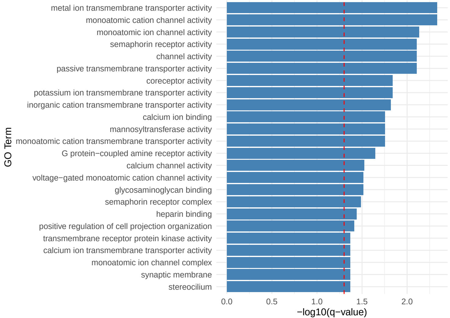
Pattern 53 Top Enriched GO Terms
