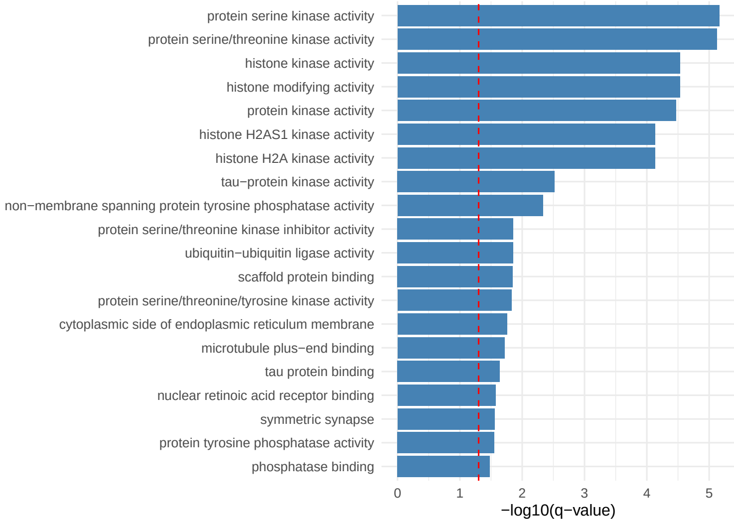
Pattern 64 Top Enriched GO Terms
