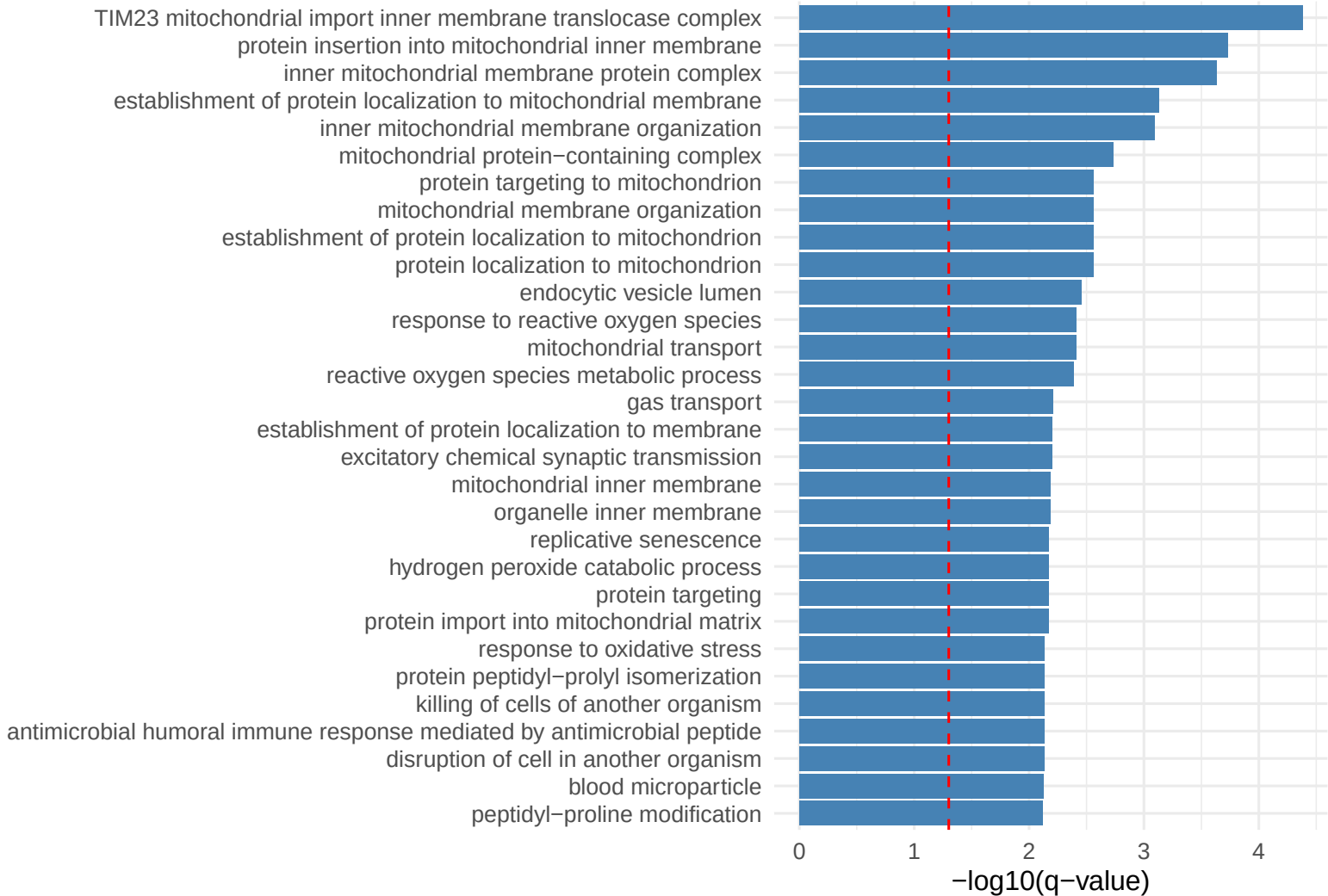
Pattern 28 Top Enriched GO Terms
