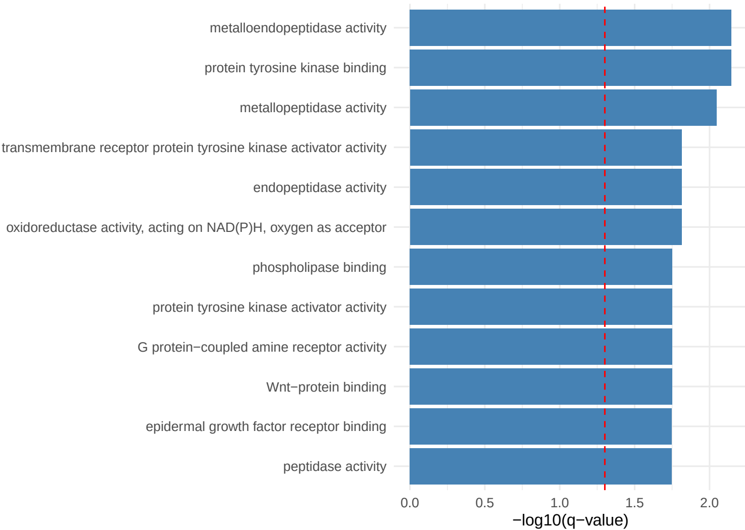
Pattern 32 Top Enriched GO Terms
