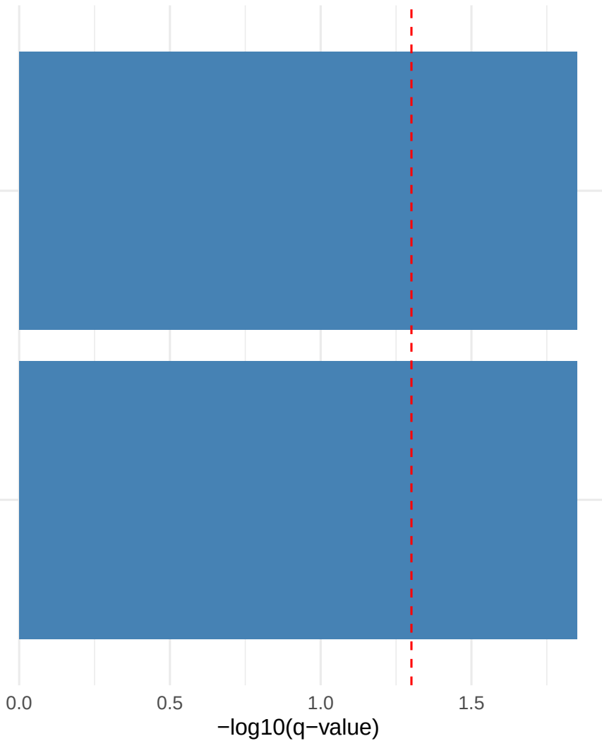
Pattern 3 Top Enriched GO Terms
