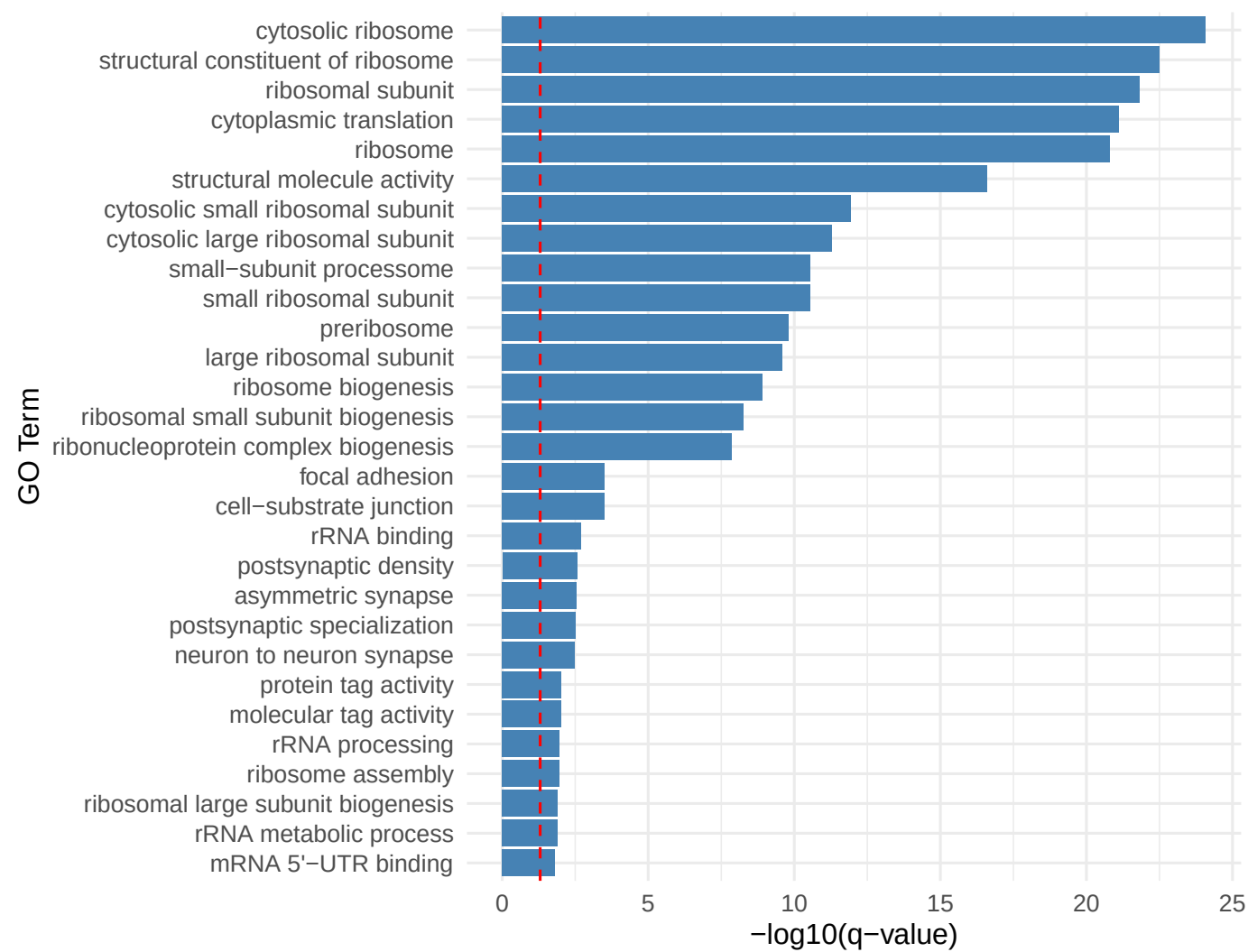
Pattern 41 Top Enriched GO Terms
