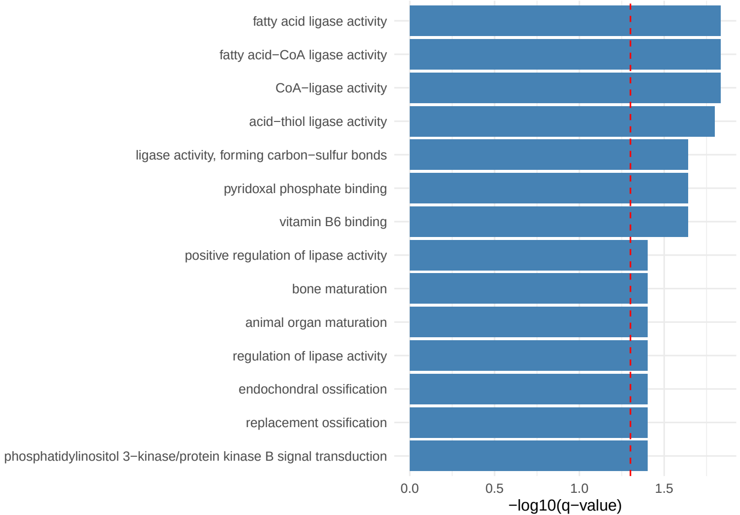
Pattern 49 Top Enriched GO Terms
