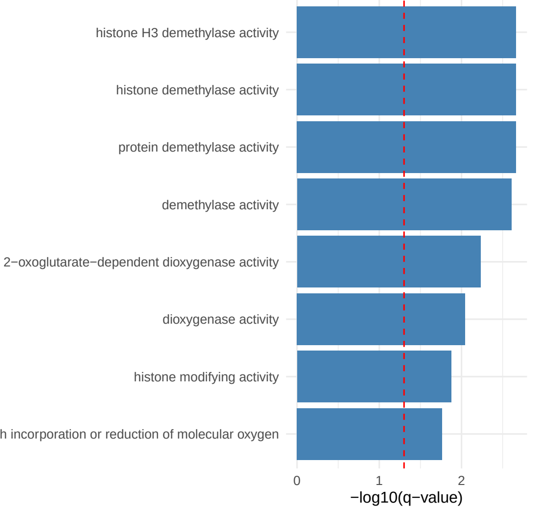
Pattern 64 Top Enriched GO Terms
