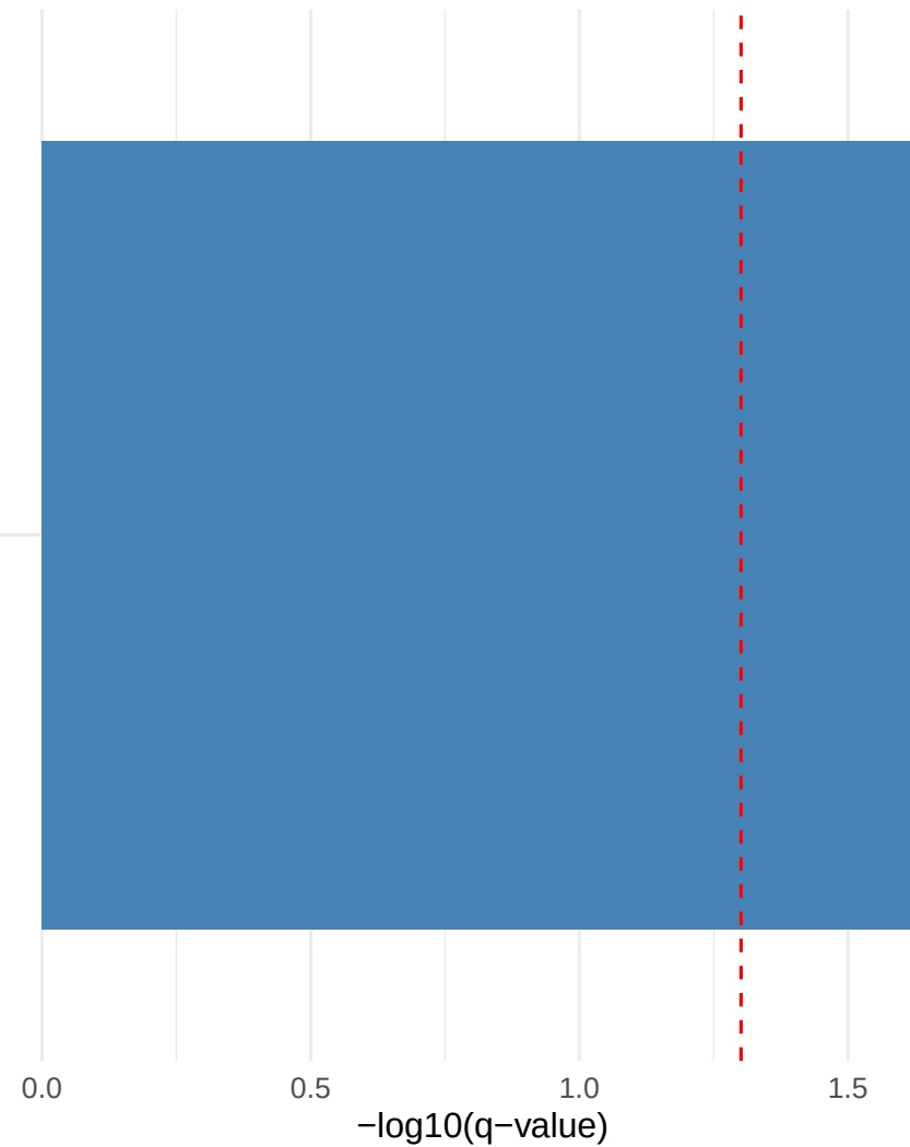
Pattern 76 Top Enriched GO Terms
