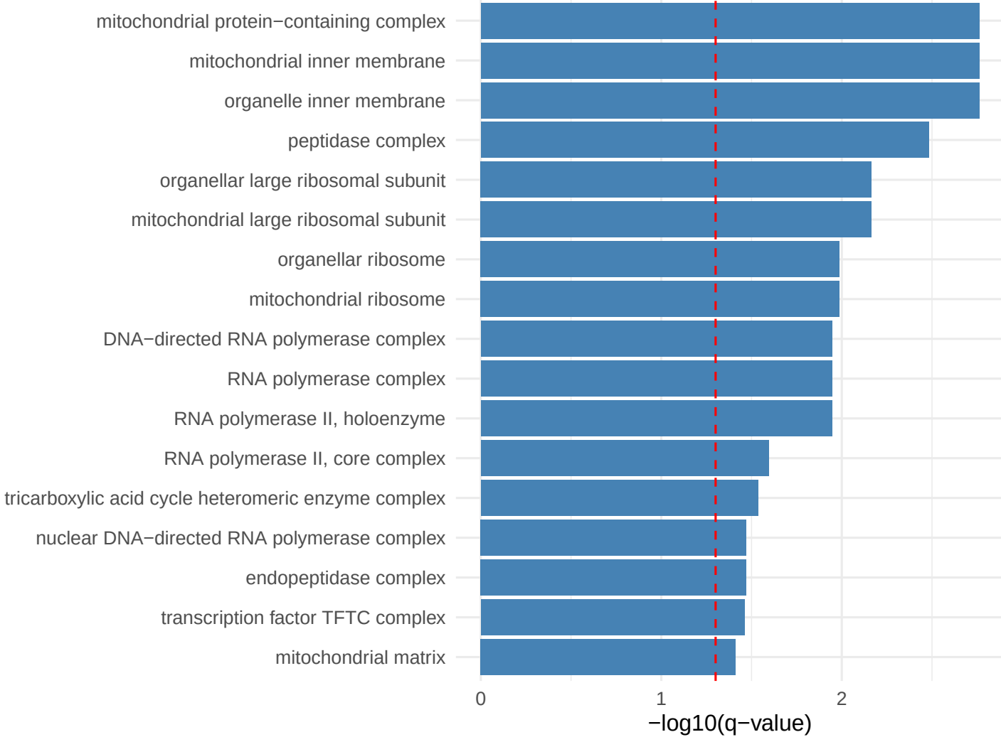
Pattern 14 Top Enriched GO Terms
